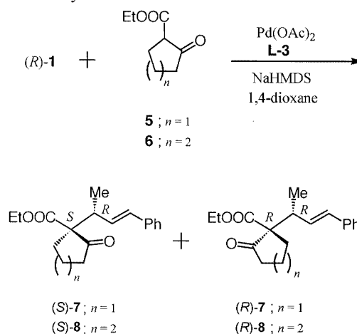
Scheme 3. Reaction of 2-ethoxycarbonylcycloketones with ( R )-1
