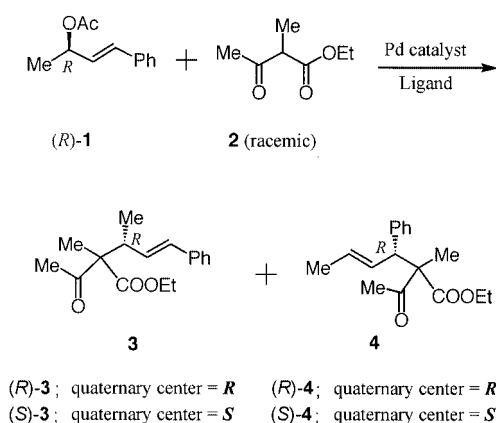
Scheme 2. Reaction of ethyl 2-methylacetoacetate with ( R )-2-acetoxy-4-phenyl-3-butene
