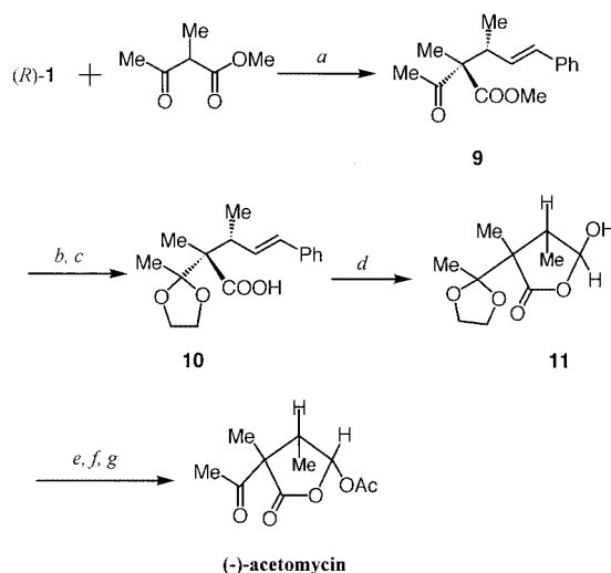
Scheme 4. Synthesis of (–)-acetomycin; reagents & conditions: a) cat. Pd(OAc) 2 , 2-(diphenylphosphanyl)naphthoic acid, NaHMDS, 1,4-dioxane; b) cat. CSA, ethylene glycol, benzene, reflux; c) LiSCl 2 H 25 , HMPA; d) O 3 , CH 2 Cl 2 , then Me 2 S; e) MsCl, Et 3 N, CH 2 Cl 2 ; f) AcOK, dibenzo-18-crown-6, toluene, reflux; g) TsOH, acetone
