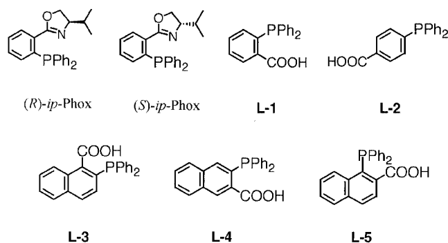
Figure 1. Structures of phosphane ligands
