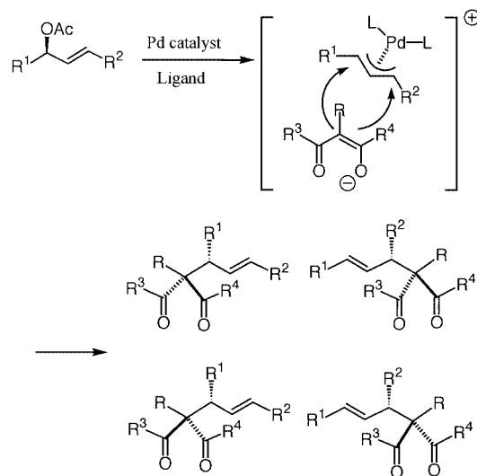
Scheme 1. Pd catalyzed allylic alkylation of \alpha -substituted \beta -diketone with chiral non-racemic allyl acetate
